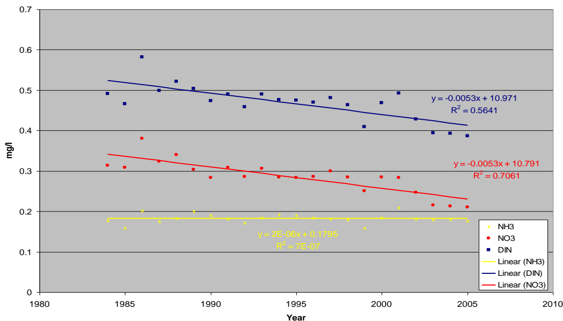
Figure L-2. Trend of estimated average \text{NO}_3 , \text{NH}_3 and DIN deposition concentrations input to the Phase 5.3 Chesapeake Bay Watershed Model.
