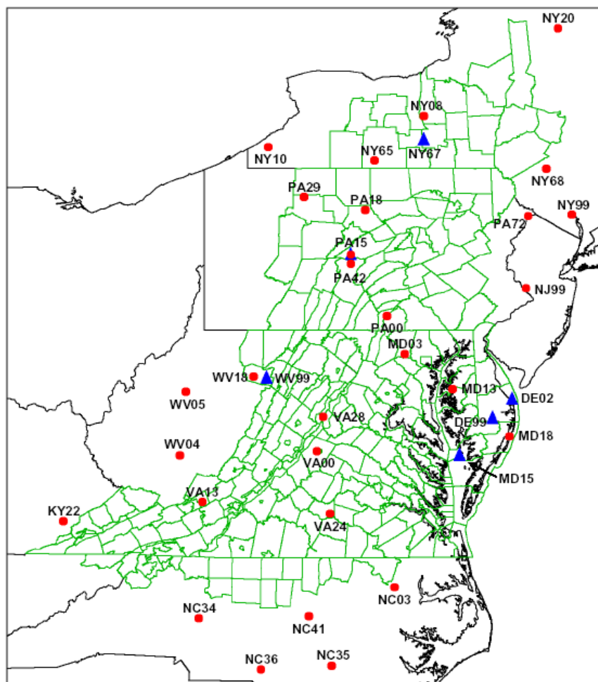
Figure L-6. Atmospheric deposition monitoring stations used in developing the wet deposition regression model.
