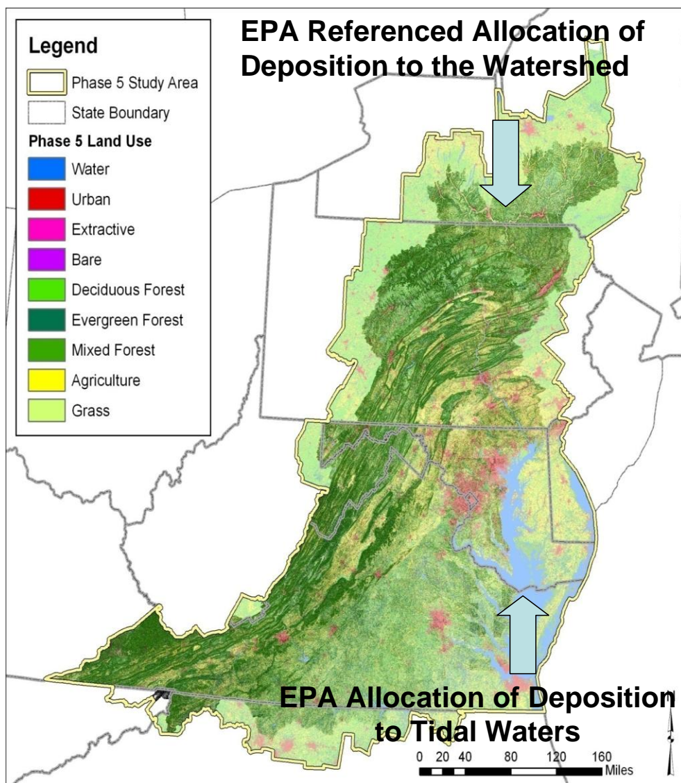
Figure L-13. EPA's reference allocation of nitrogen atmospheric deposition to the Bay watershed and the allocation of nitrogen atmospheric deposition direct to tidal waters.
