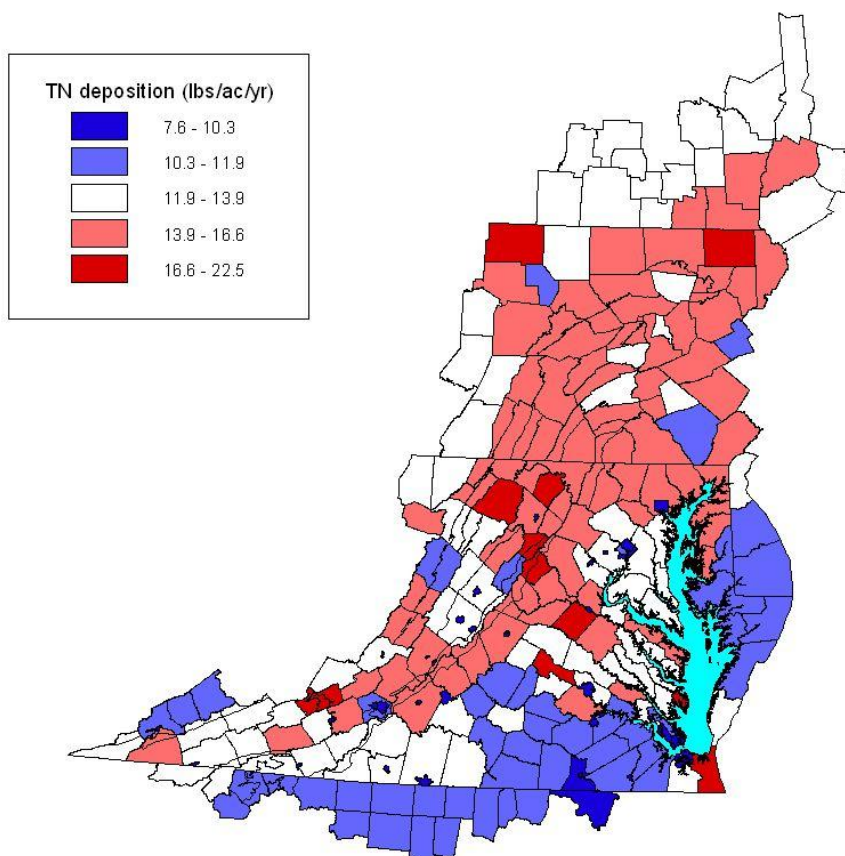
Figure L-8. Annual average DIN atmospheric deposition on land segments in the entire Phase 5.3 Chesapeake Bay Watershed Model domain.
