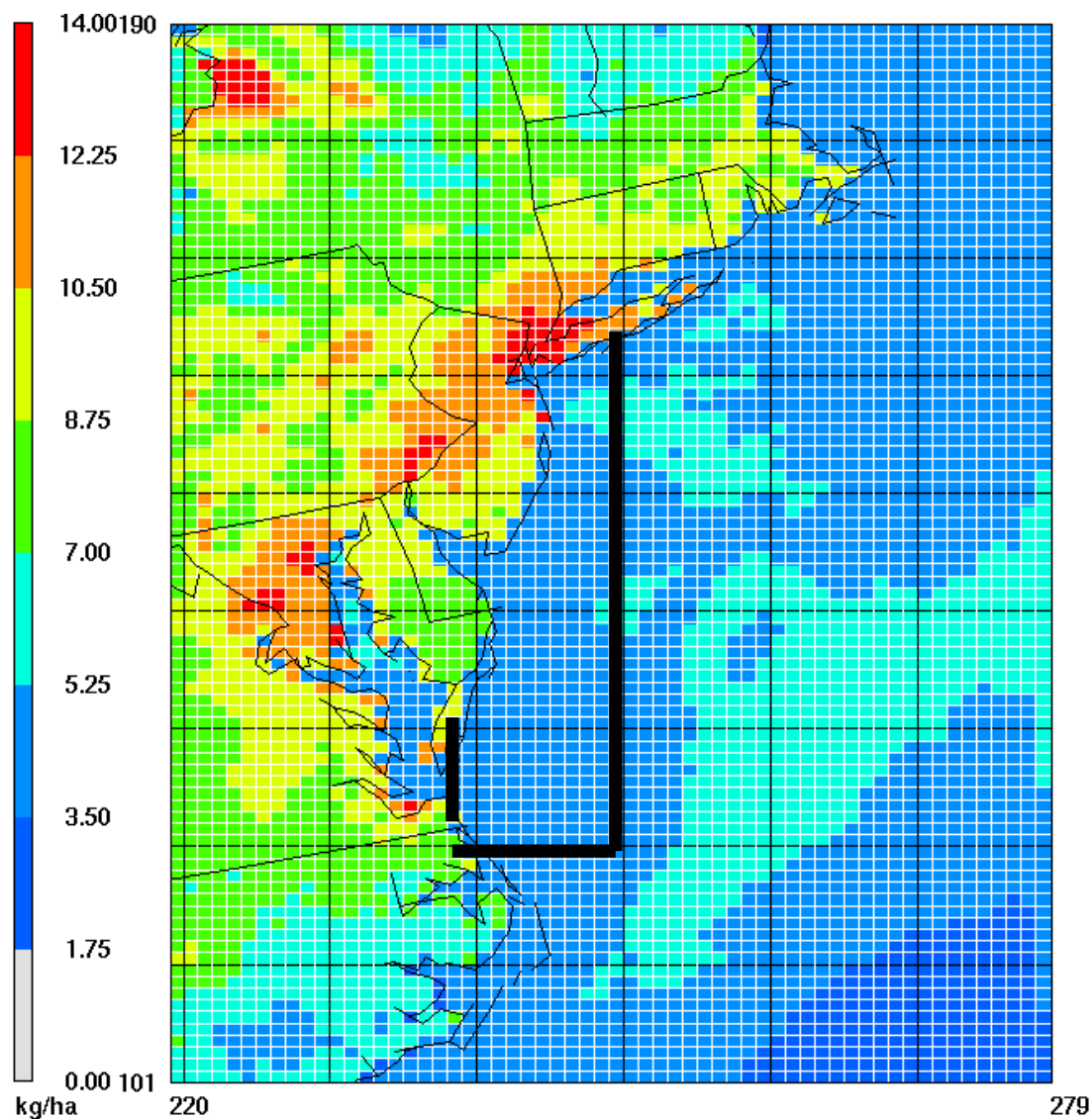
Figure L-11. Boundaries of the coastal ocean region used to adjust the ocean boundary conditions in the Chesapeake Bay WQSTM.
