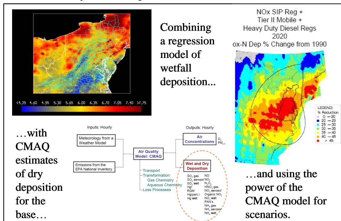
Figure L-5. The Chesapeake Bay Airshed Model is a combination of a regression model of wet deposition and the CMAQ model of dry deposition.
