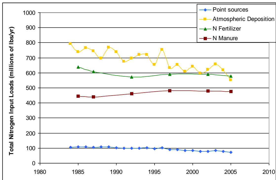
Figure L-1. 20-year (1985–2005) time series of atmospheric, fertilizer, manure, and point source nitrogen input loads to the Chesapeake Bay Water Quality and Sediment Transport Model.
